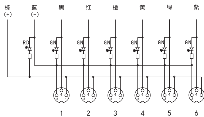
S010-M8-6P S011-M8-6P
