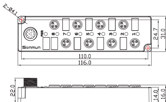
S011-M8-8P/8C
