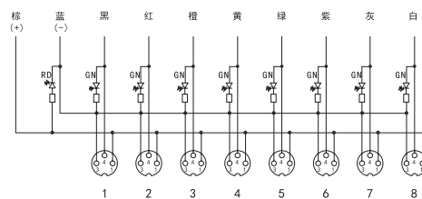
S010-M8-8P S011-M8-8P
