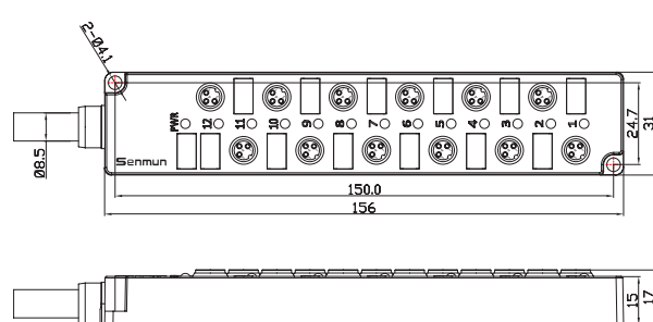
S010-M8-12/12P/12C
