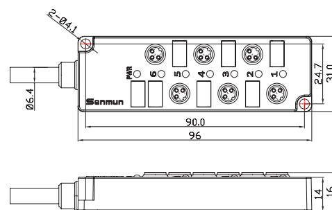
S010-M8-6/6P/6C
