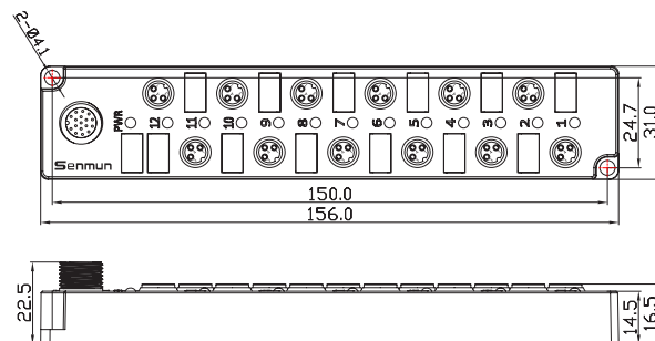
S011-M8-12/12P/12C
