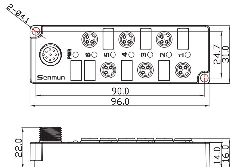
S011-M8-6/6P/6C
