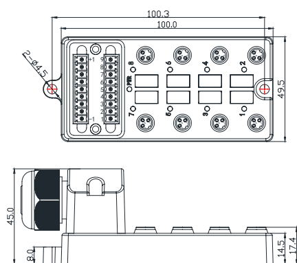
S012-M8-8P/8C
